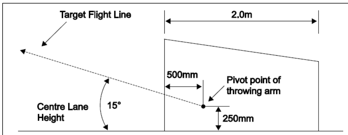
Diagram 5.1 Trap Construction
