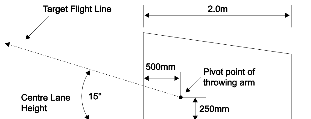
Diagram 5.1 Trap Construction
