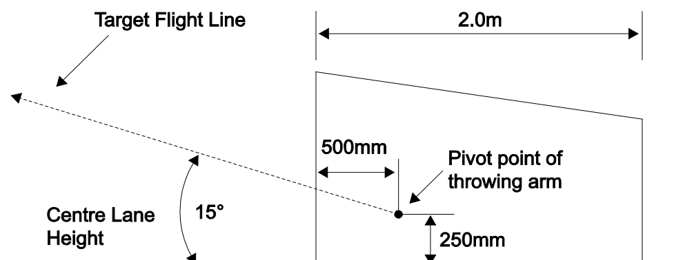
Diagram 5.1 Trap Construction
