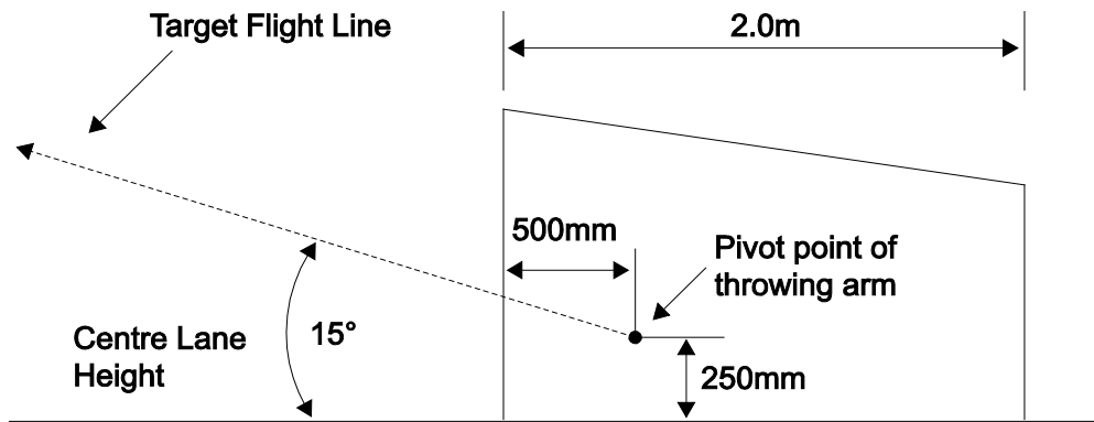
Diagram 5.1 Trap Construction
